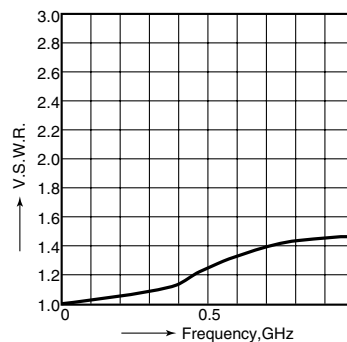
11.-(3) High-frequency characteristics V.S.W.R.
