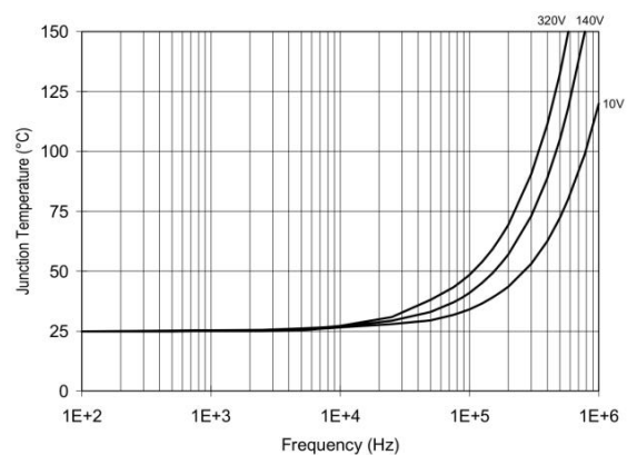
Figure 34. XL2110S/XL2113S TJ vs. Frequency (IRFBC40) RGATE = 15Ω, VCC = 15V
