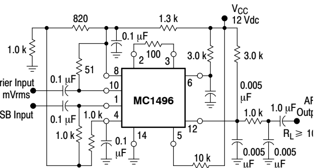
Figure 28. Product Detector (12 Vdc Single Supply)
