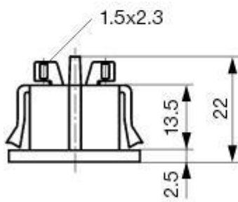
Solder terminals for wires
